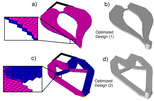
Fig. 2. Optimized designs obtained by topology optimization. (a) and (c): MATLAB FEM, (b) and (d): COMSOL implementation
