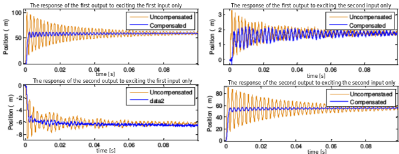
Figure 4- Exciting one input and showing the cross coupling effect – experimental
