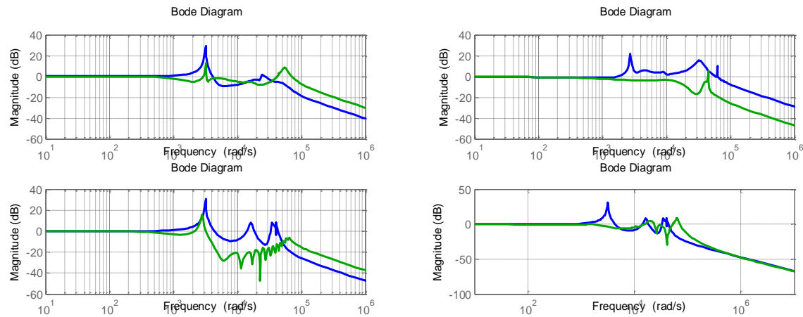
Figure 7- Compensated and un-compensated system frequency responses
