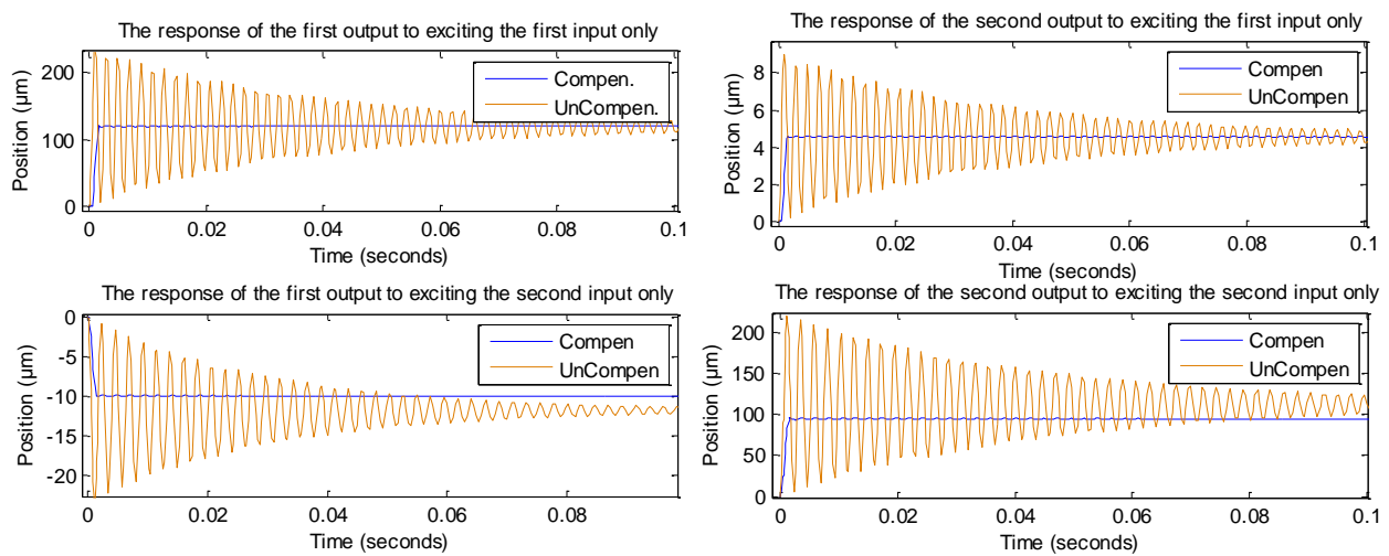
Figure 3- Exciting one input and showing the cross coupling effect – simulation
