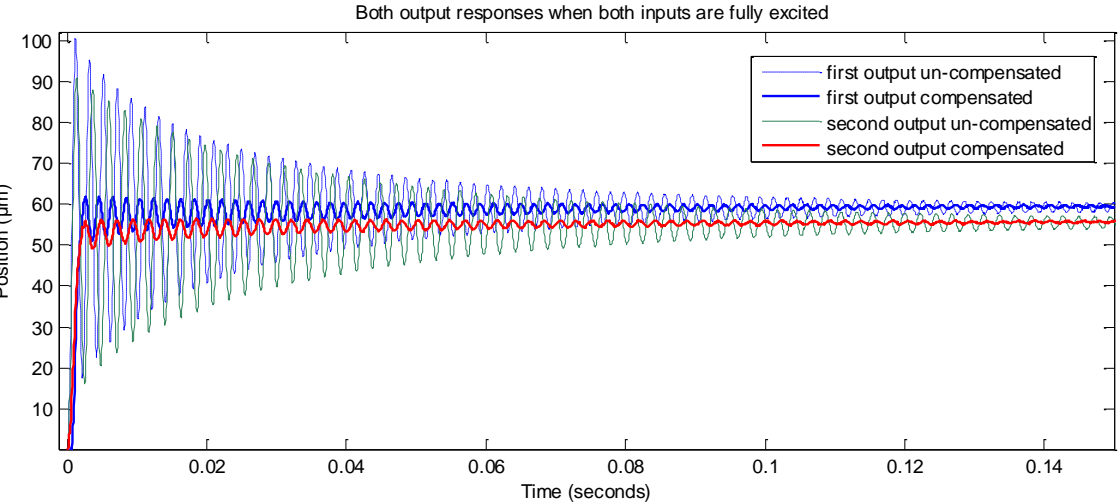
Figure 6- Exciting both inputs and showing both outputs, compensated and non-compensated – experimental
