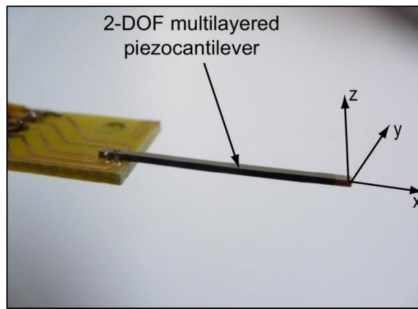
Figure 1: The two degrees of freedom (2-DOF) piezoelectric micropositioner.
