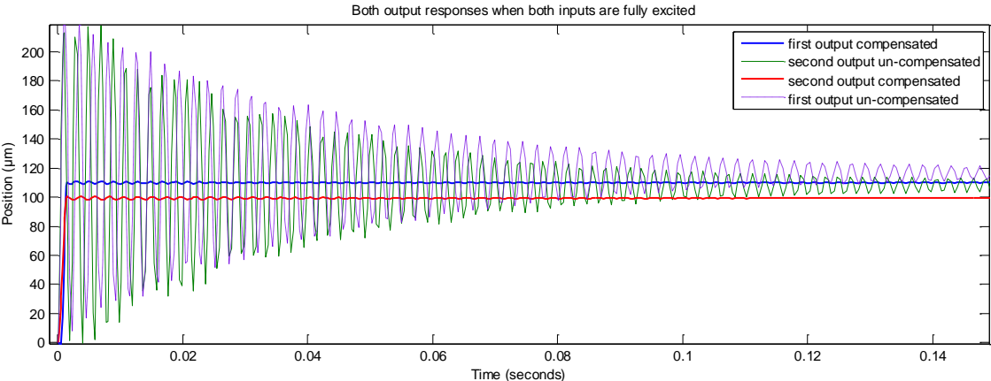
Figure 5- Exciting both inputs and showing both outputs, compensated and non-compensated - simulation
