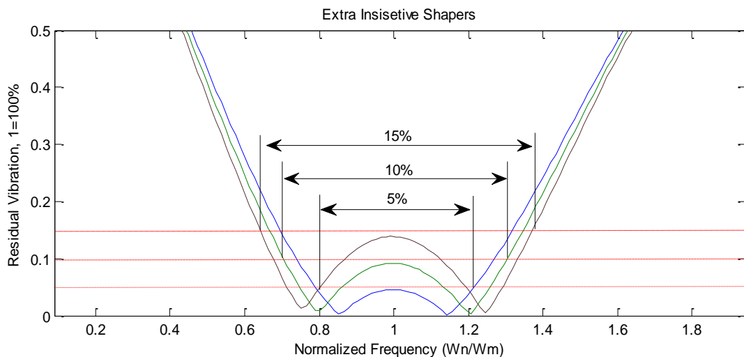
Figure 9: EI shapers sensitivity curves - Simulation
