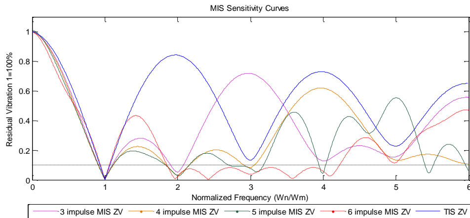
Figure 14: MIS ZV shapers sensitivity curves – wider range - Simulation
