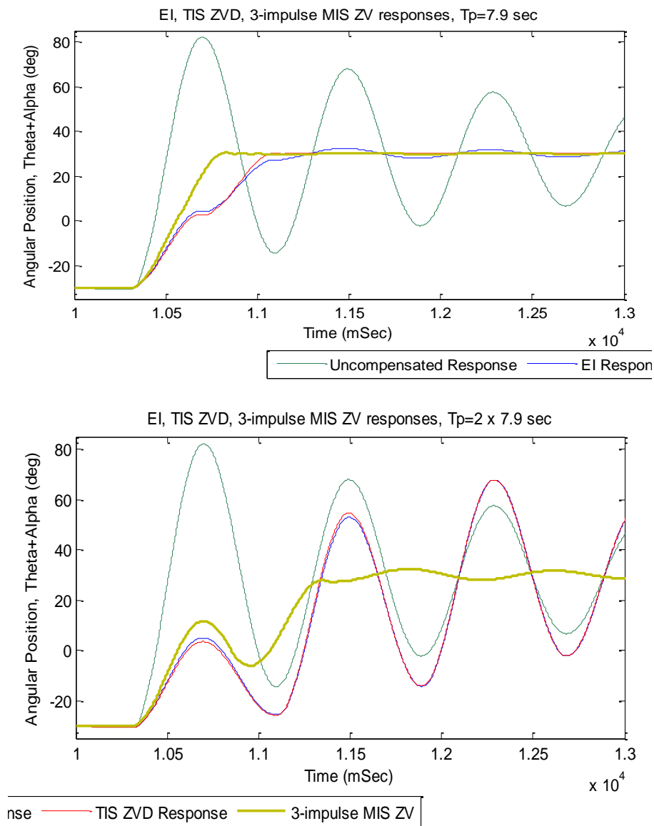
Figure 16: \theta + \alpha 3-Impulse MIS ZV, EI, and TIS ZVD Responses – Experimental
