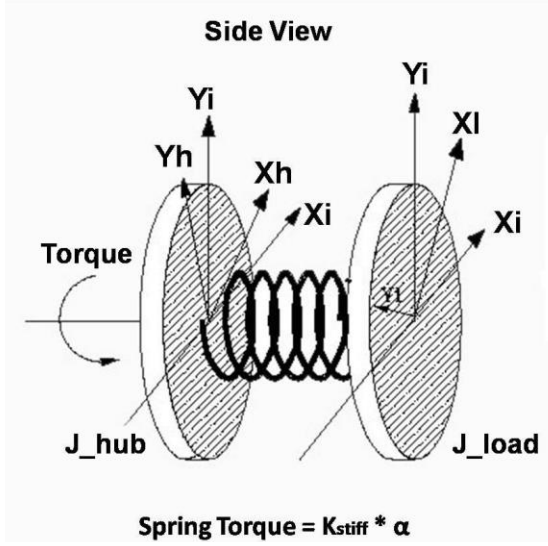
Figure 3: Simplified Model
