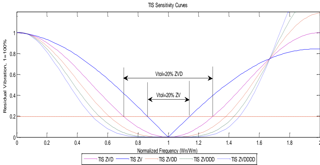
Figure 8: TIS Sensitivity Curves – Simulation
