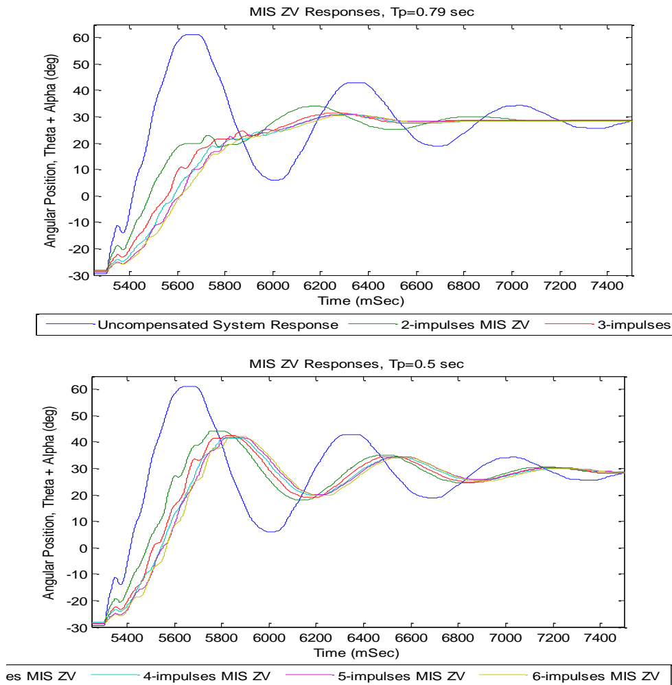
Figure 7: MIS ZV Responses – Experimental
