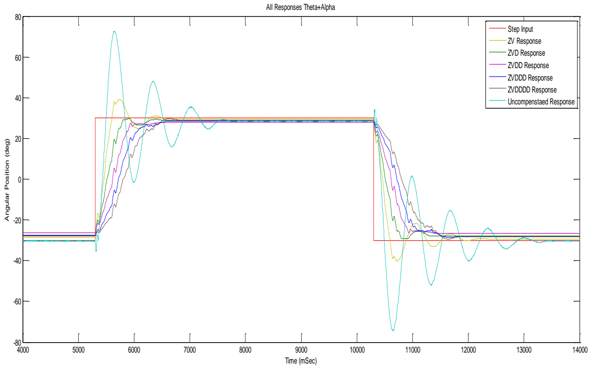
Figure 4: Tip Responses – TIS Experimental
