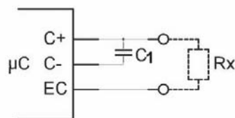
Figure 1: Basic measurement schematic
