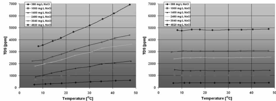
Figure 11 - Non-compensated model TDS to temperature characteristic. Figure 12 - Compensated model TDS to temperature characteristic (various concentrations).
