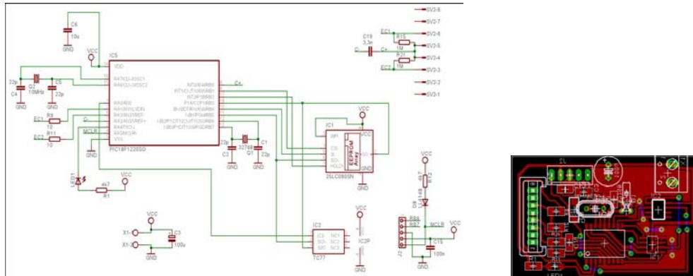
Figure 7: Schematic of the second temperature compensated model. Figure 8: Printed circuit board.
