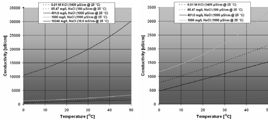
Figure 9 - Conductivity to temperature characteristics for different concentrations. Figure 10 - Same graph re-scaled.
