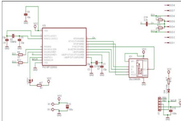
Figure 5: Schematic of the first uncompensated model.
