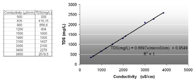
Figure 4: TDS measured by device versus conductivity measured by the referencing device (in a mixture of KCl+NaCl solutions at 20 °C).
