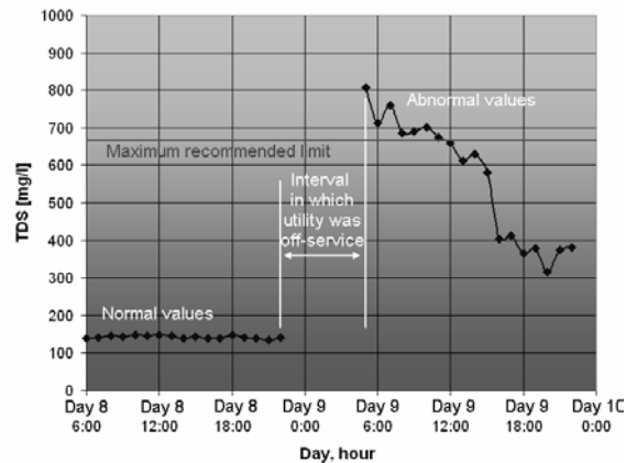
Figure 14 - Abnormal fluctuation due to the water utility shutdown between 23:00 and 5:00.
