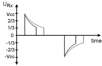
Figure 2: Electrodes signal waveforms for two different water conductivities
