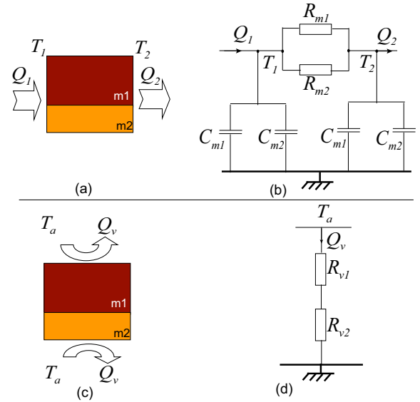
Fig. 8. Parallel and serial thermal structures.
