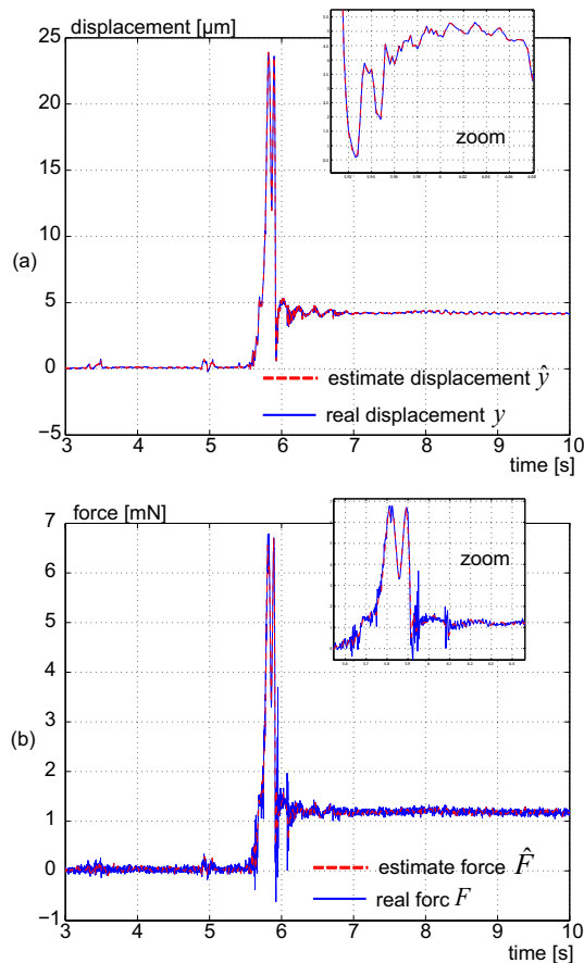
Fig. 7. Experimental validation with F \neq 0mN (actuator in contact with the force sensor).
