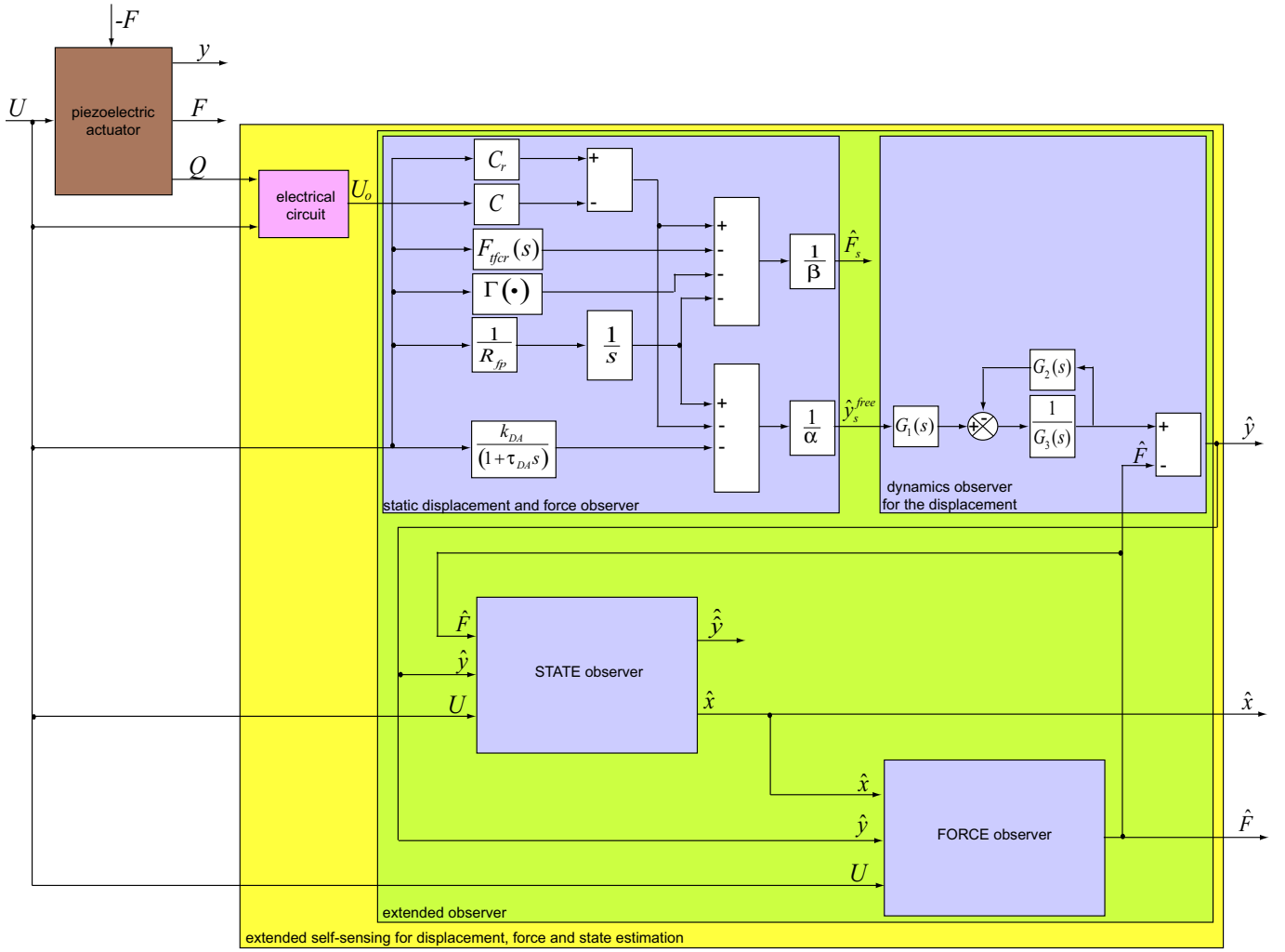
Fig. 4. Principle scheme of the extended complete self-sensing.
