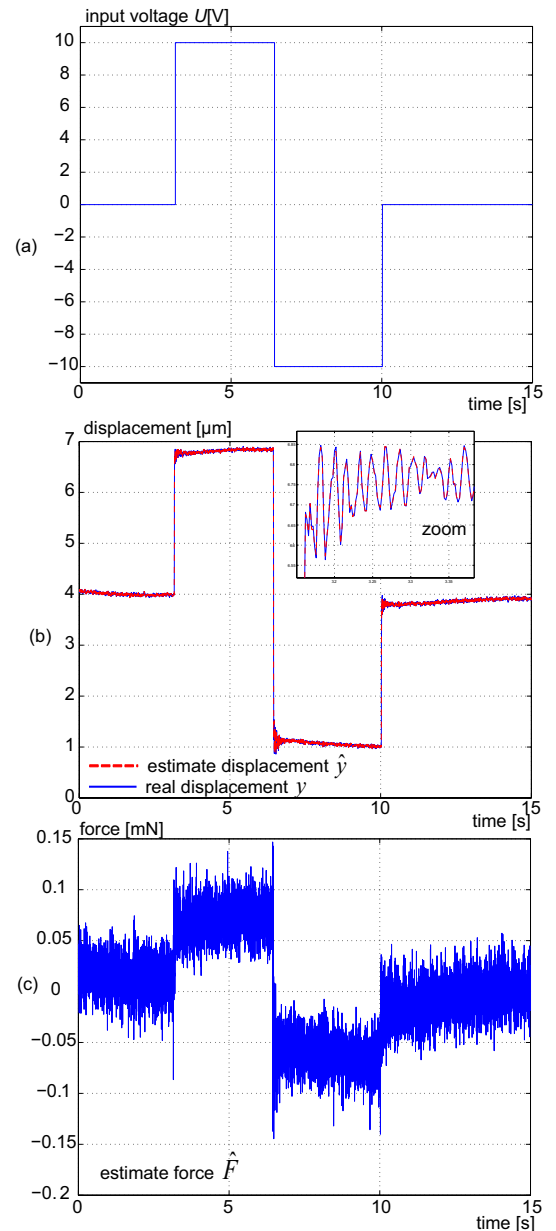
Fig. 6. Experimental validation with F = 0mN (actuator in free condition).
