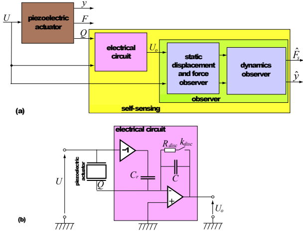
Fig. 2. Complete self-sensing [5]: (a) - principle scheme. (b) - electrical circuit used.
