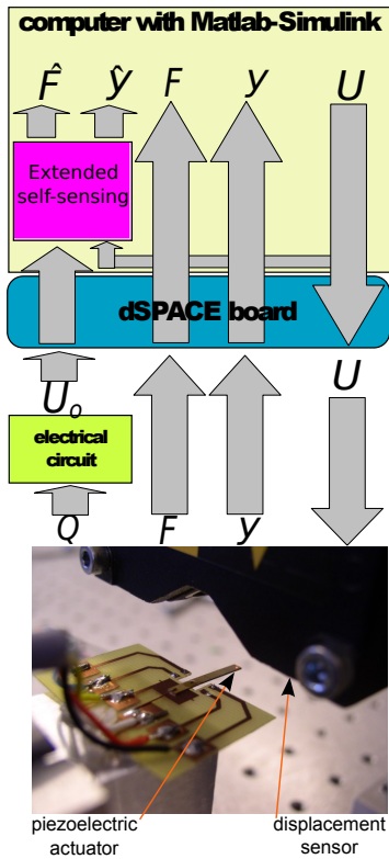
Fig. 5. The experimental setup.
