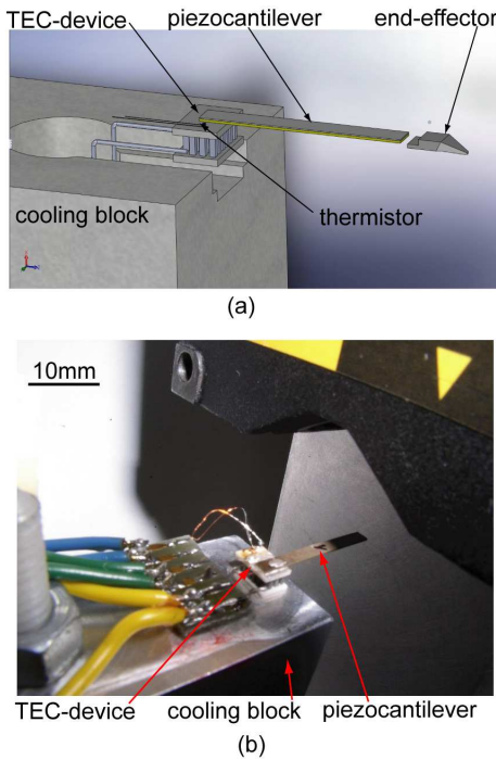
Fig. 1. CAD-drawing (a) and a photograph (b) of the thermo-piezoelectric cantilever.
