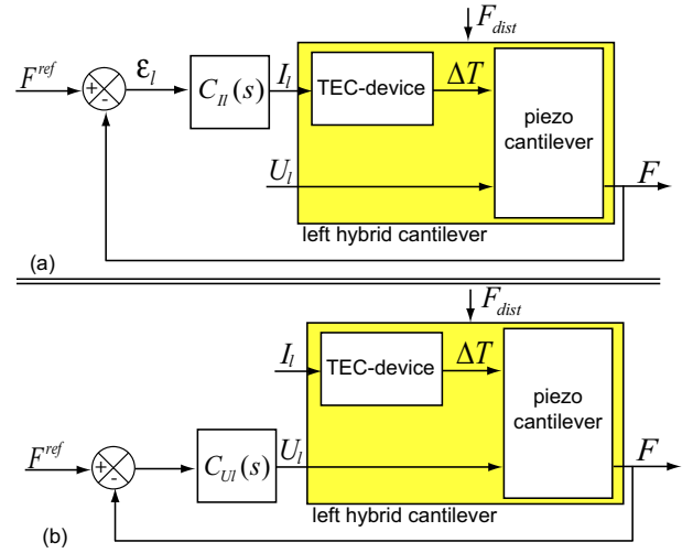
Fig. 14. Closed-loop scheme (a) for the coarse mode, (b) for the fine mode.
