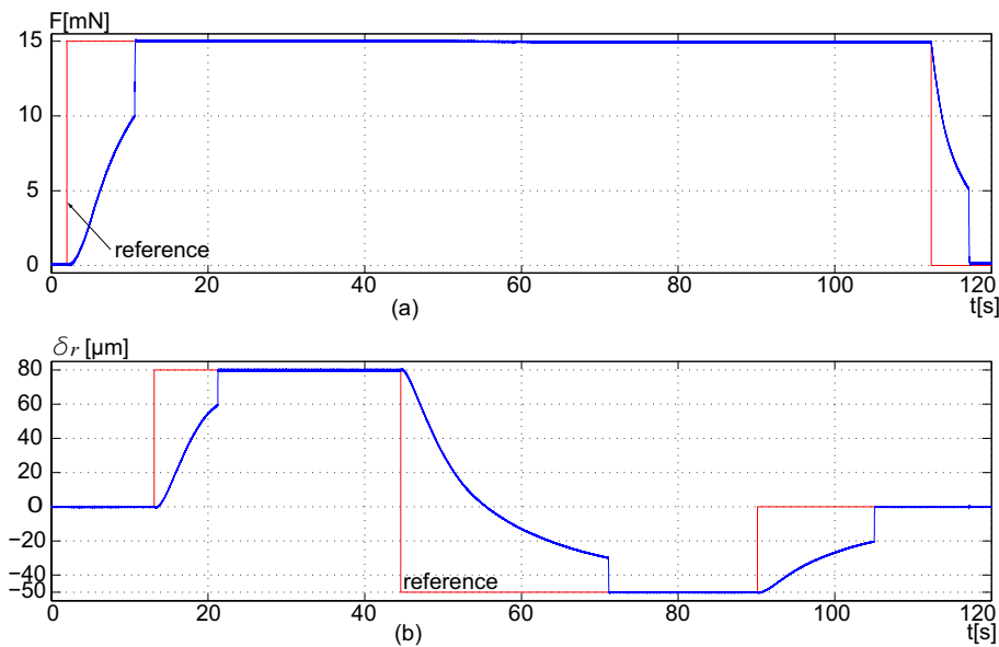
Fig. 19. Experimental result of an controlled pick-and-place task with controlled position and force: (a) reference and measured output manipulation force (from the left cantilever), (b) reference and measured output position (from the right cantilever).
