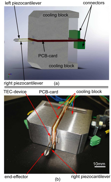
Fig. 2. CAD-drawing (a) and a photograph (b) of the hybrid thermo-piezoelectric microgripper [20].
