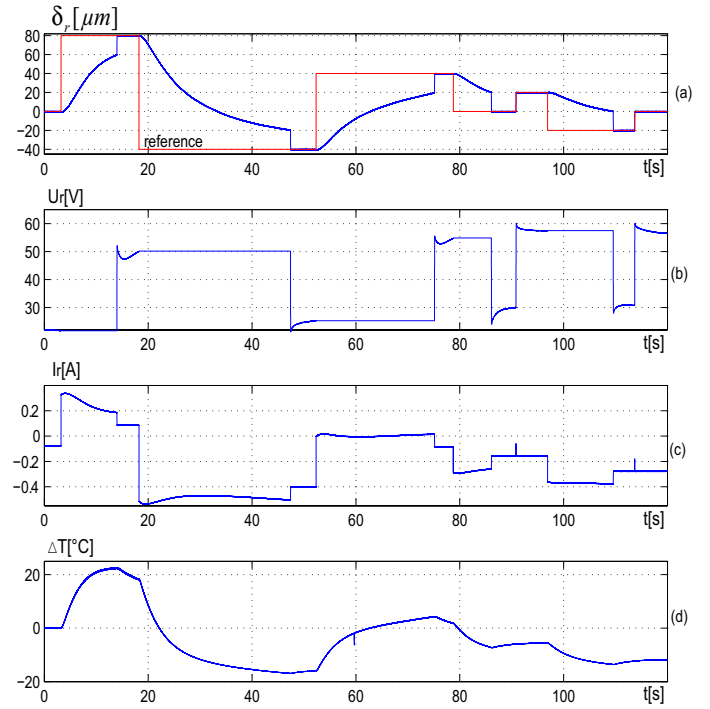
Fig. 9. Step response of the closed-loop hybrid cantilever: (a) reference and measured output deflection, (b) applied voltage, (c) applied electric current to the TEC-device, (d) measured temperature difference.
