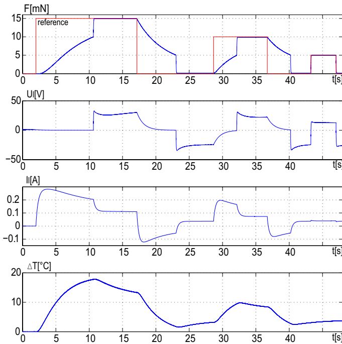
Fig. 16. Response of the closed-loop hybrid cantilever: (a) reference and measured output force, (b) applied voltage, (c) applied electric current to the TEC-device, (d) measured temperature difference.
