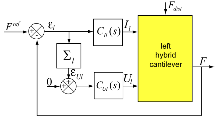
Fig. 15. Complete control scheme of the left hybrid cantilever.
