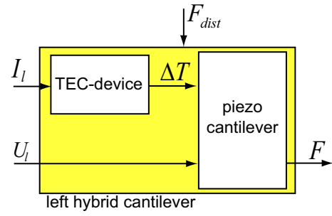
Fig. 11. Systemic scheme of the left hybrid cantilever.
