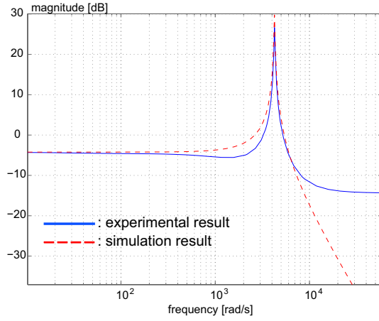
Fig. 13. Harmonic response of the piezoelectric part: experimental result and model simulation.
