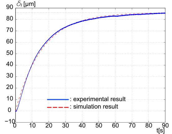
Fig. 12. Step response of the electro-thermomechanical part: experimental result and model simulation.
