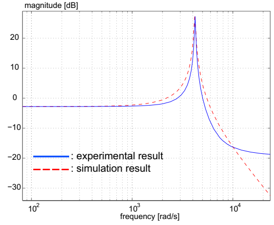
Fig. 6. Harmonic response of the piezoelectric part: experimental result and model simulation.
