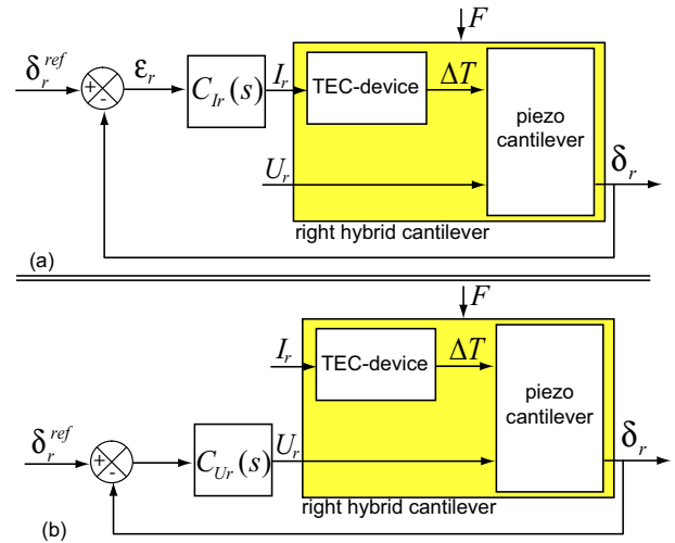
Fig. 7. Closed-loop scheme (a) for the coarse positioning mode (electro-thermomechanical functioning), (b) for the fine mode (piezoelectric functioning).
